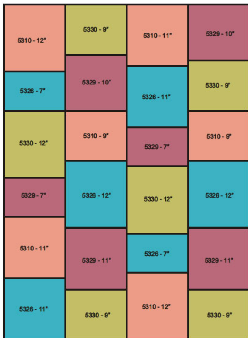
LEWIS DIAGRAM
